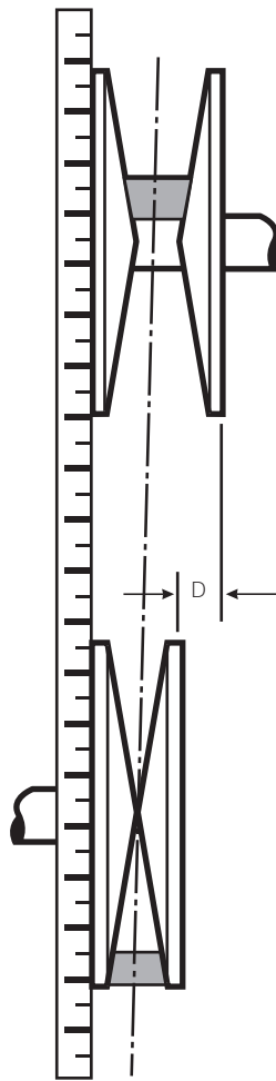
WRONG Check for misalignment and offset distance "D"
