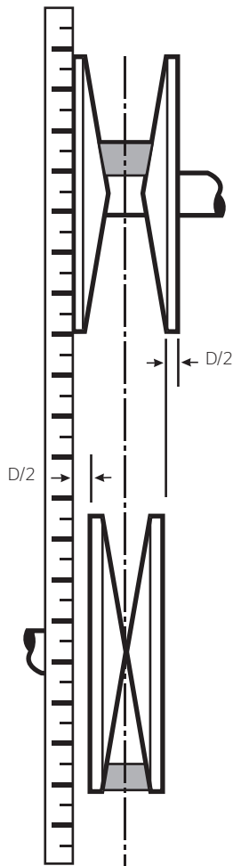
RIGHT The belt is parallel to the straight edge
